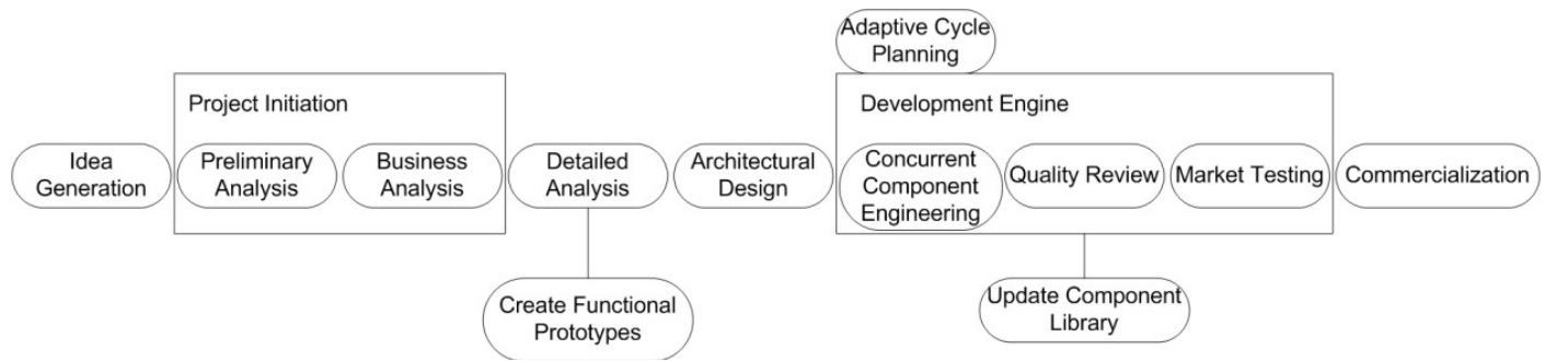
Fig. 6 Mobile development method proposed in (Rahimian & Ramsin, 2008) [5]
